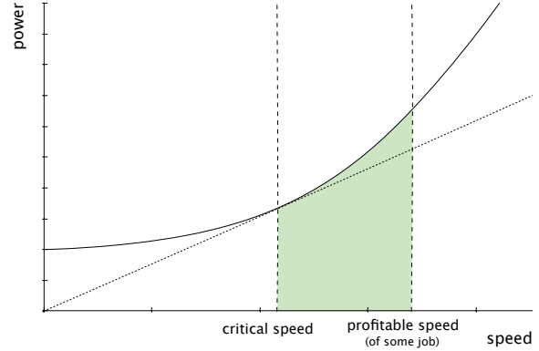
Figure 2. Our algorithm tries to use job speeds that essentially stay in the shaded interval.
